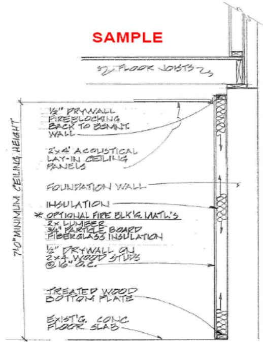
WALL SECTION
