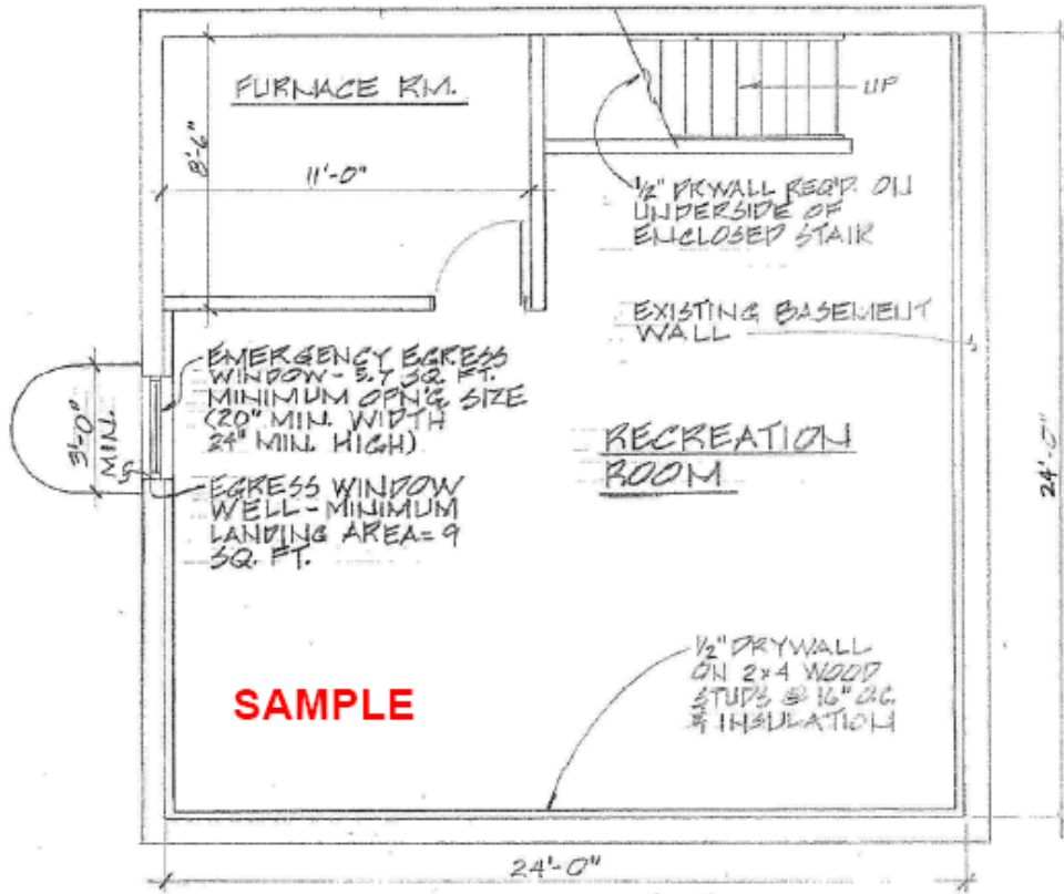
BASEMENT PLAN
